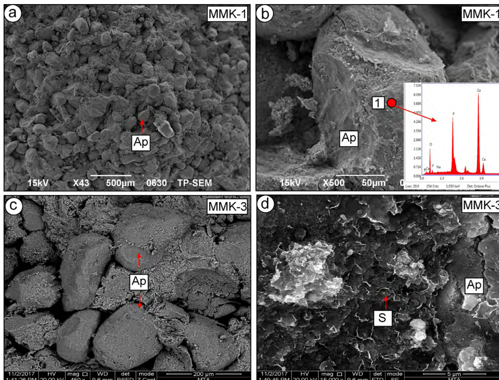
Fig. 6. SEM microphotographs of the Karababa Formation members phosphorite rocks
