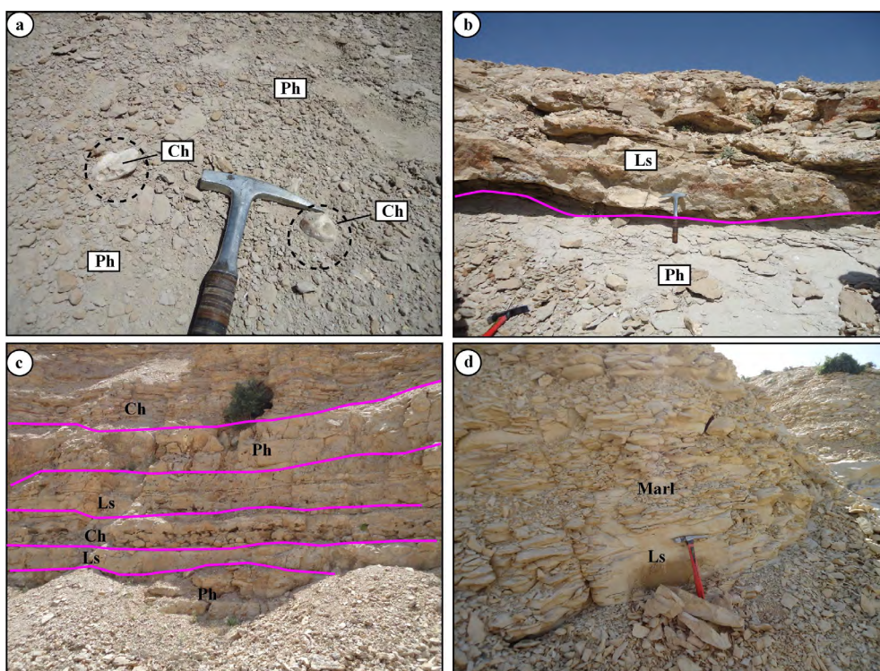
Fig. 4. Field views of the members of the Karababa Formation
