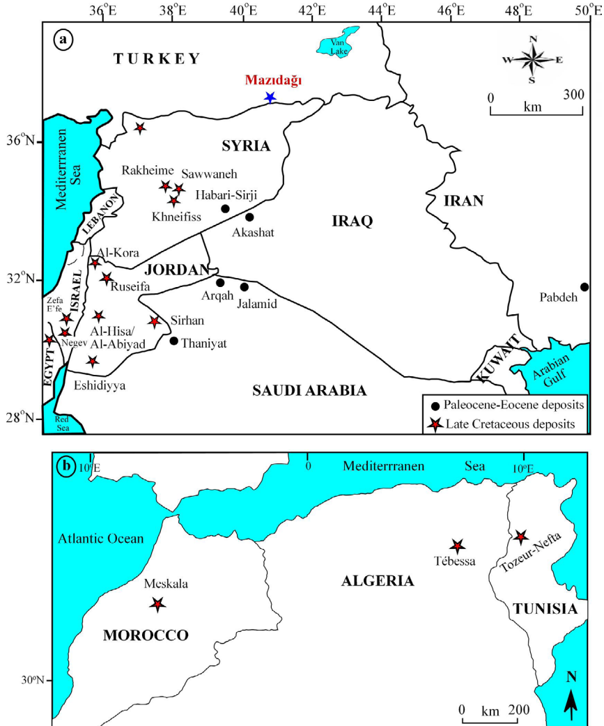
Fig. 1. Location map of the phosphorite deposits in the Mediterranean belt and adjacent countries
