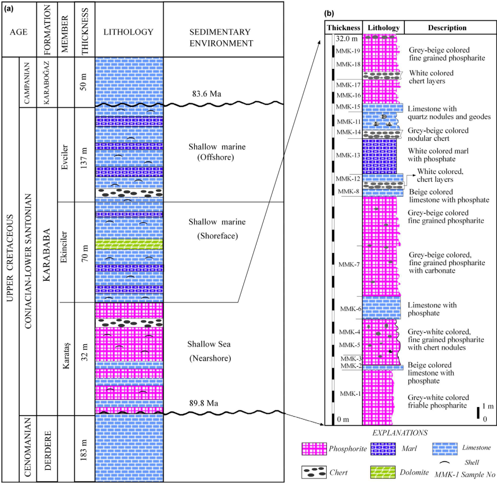
Fig. 3. a) The stratigraphic column, which is based on the measured sections, shows the interpreted sedimentary environments of the members of the Karababa Formation (Upper Cretaceous);
