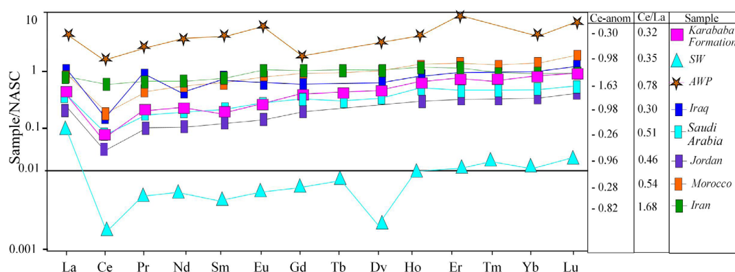
Fig. 11. NASC-normalized REE patterns of the Mazıdağı phosphorites (average value, n = 11 ), seawater (SW; Høgdahl et al. 1968), AWP (Altschuler 1980), Arabian plate countries and other composition
